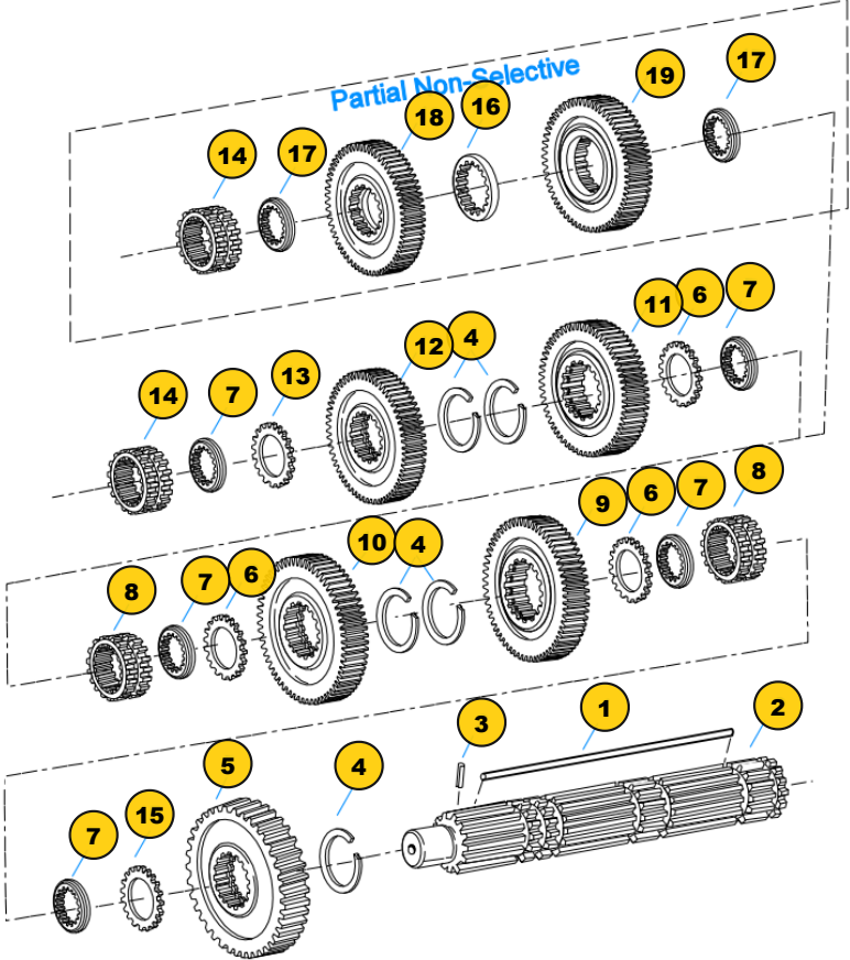
Group: MAINSHAFT ASSY
