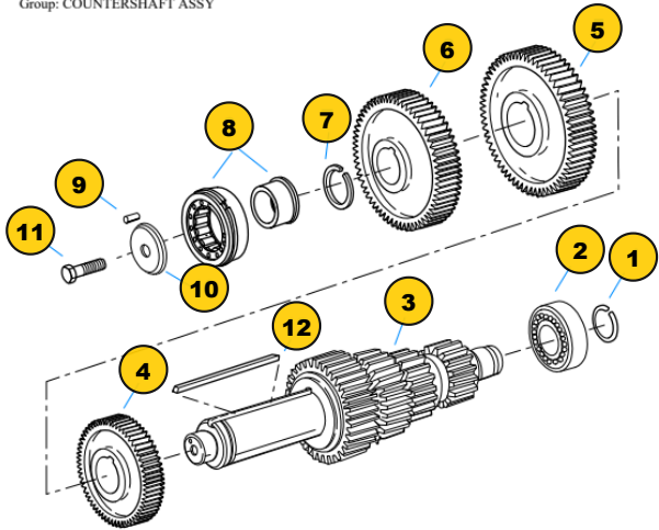
Group: COUNTERSHAFT ASSY
