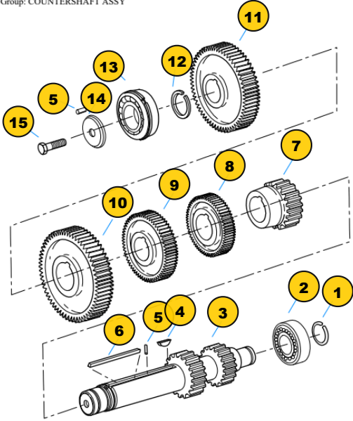
Group: COUNTERSHAFT ASSY
