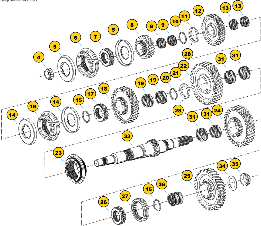
Group: MAINSHAFT ASSY
