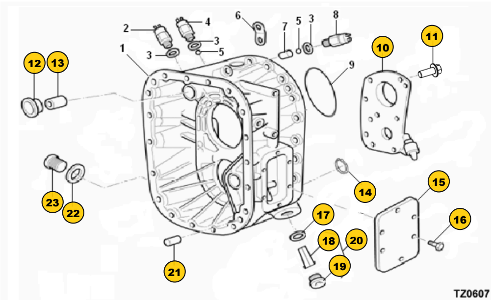
Group: INTERMEDIATE CASE ASSY.
