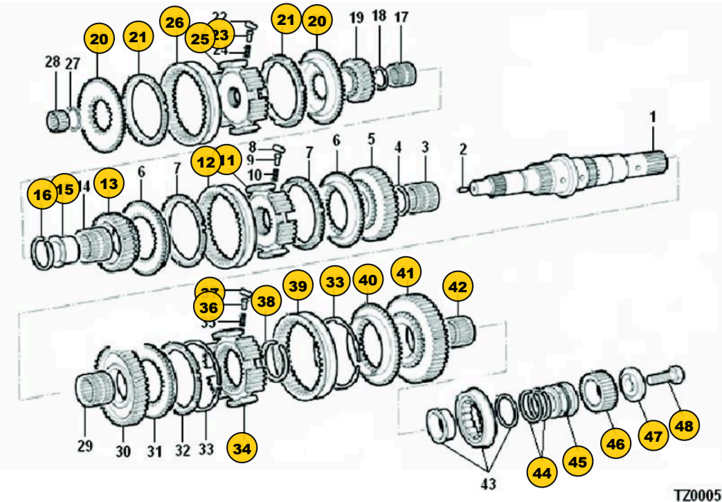
Group: MAINSHAFT ASSY.
