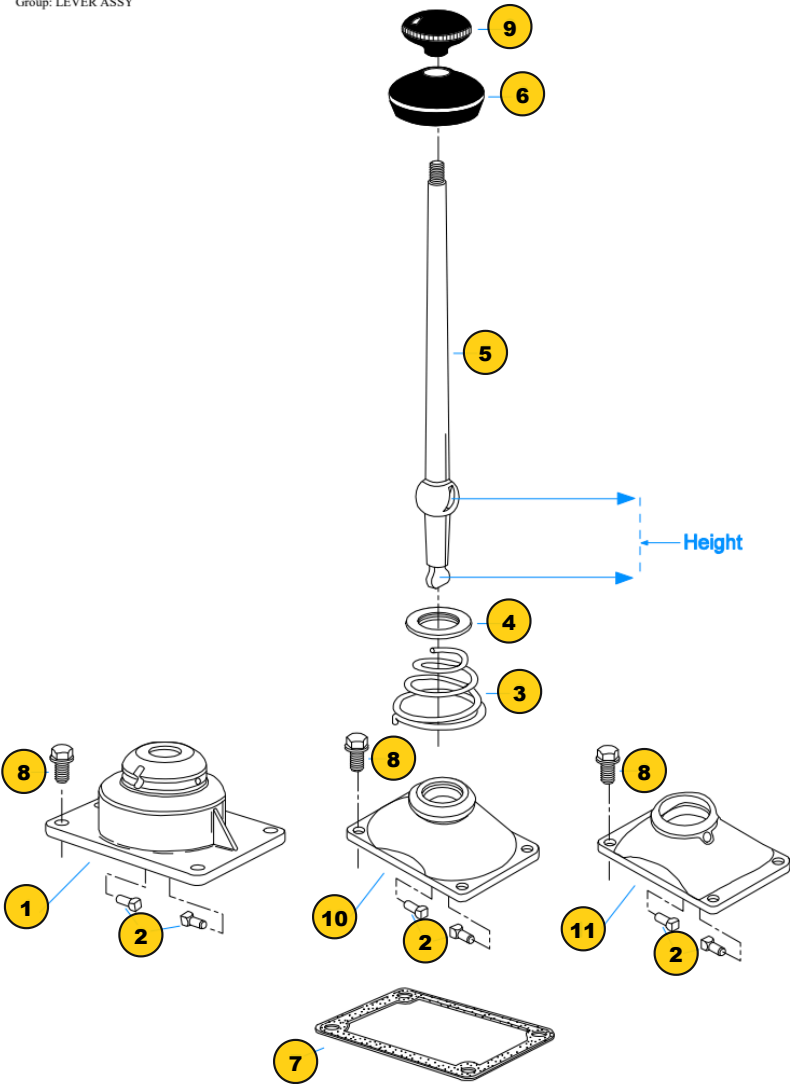
Group: LEVER ASSY
