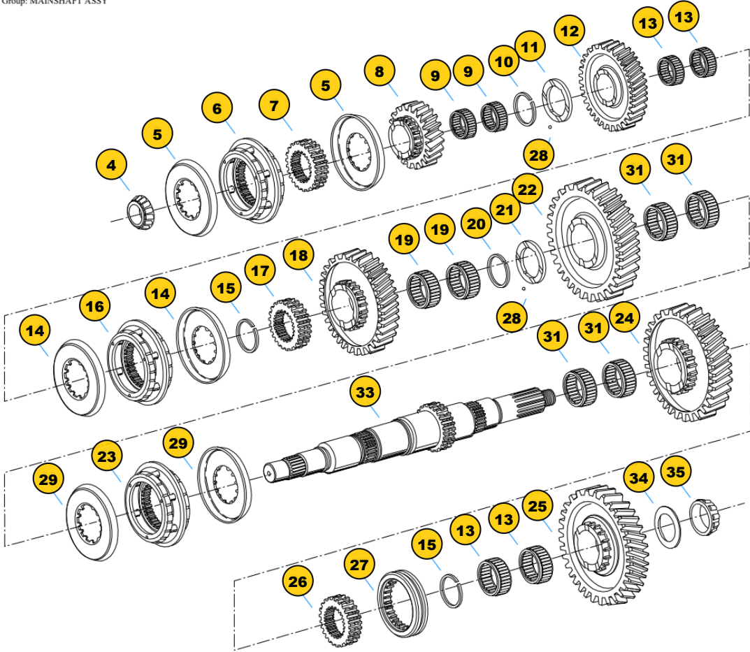
Group: MAINSHAFT ASSY
