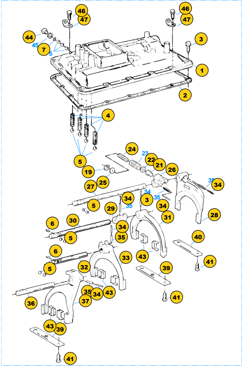
Group: SHIFT BAR HOUSING
