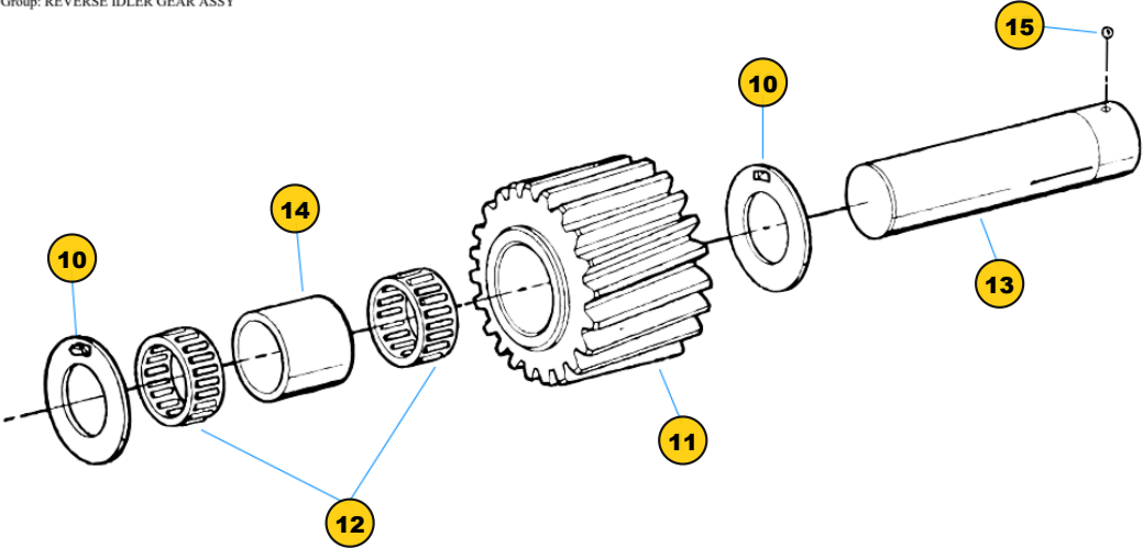
Group: REVERSE IDLER GEAR ASSY
