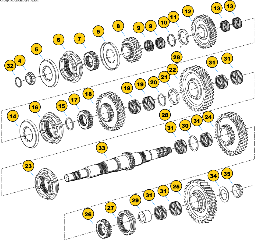
Group: MAINSHAFT ASSY
