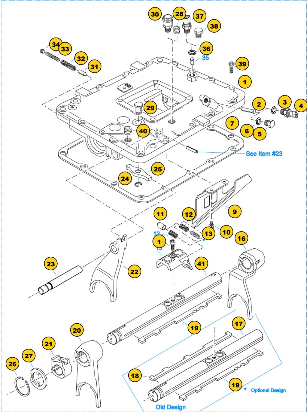
Group: SHIFT BAR HOUSING (FROF)
