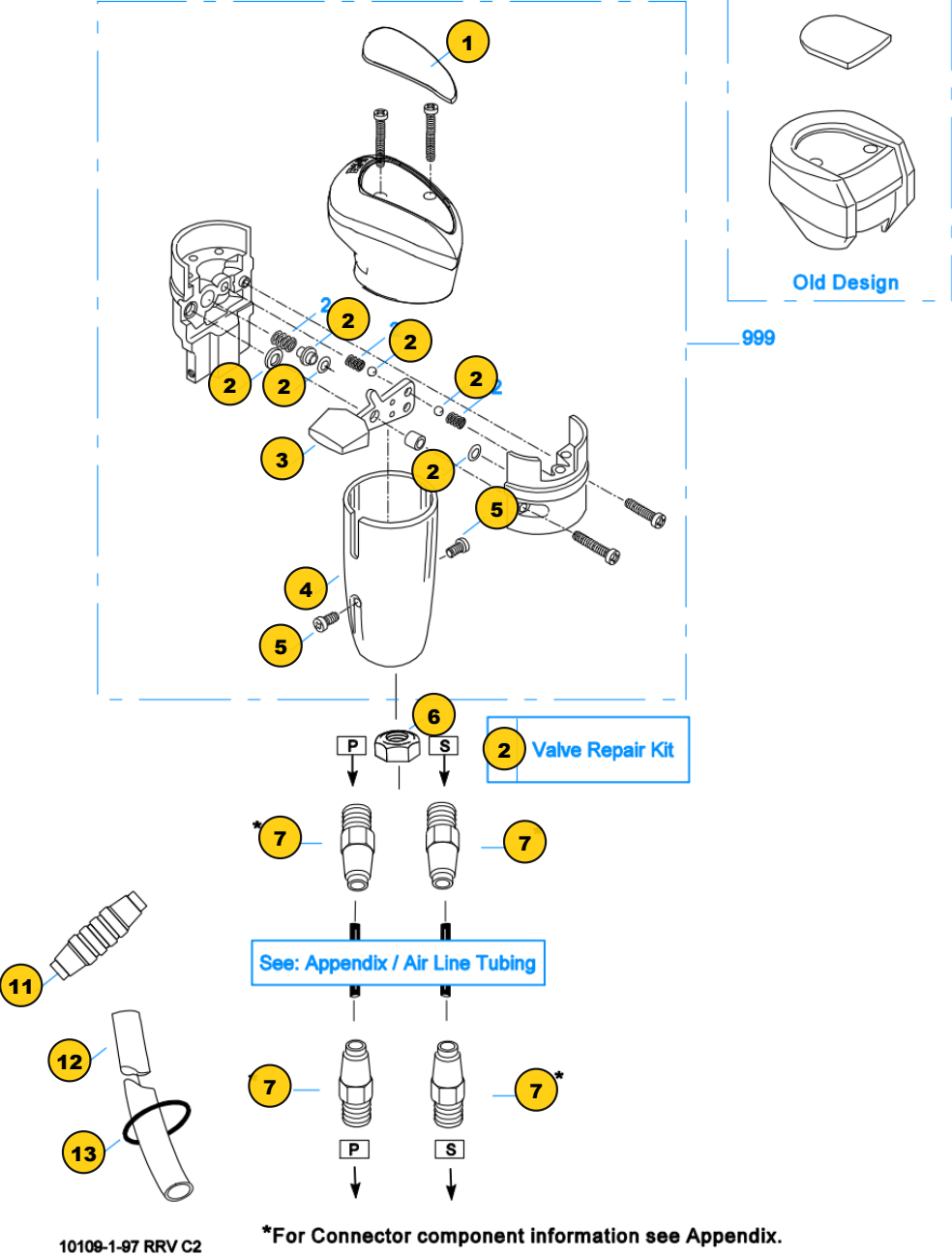
Group: ROADRANGER VALVE
