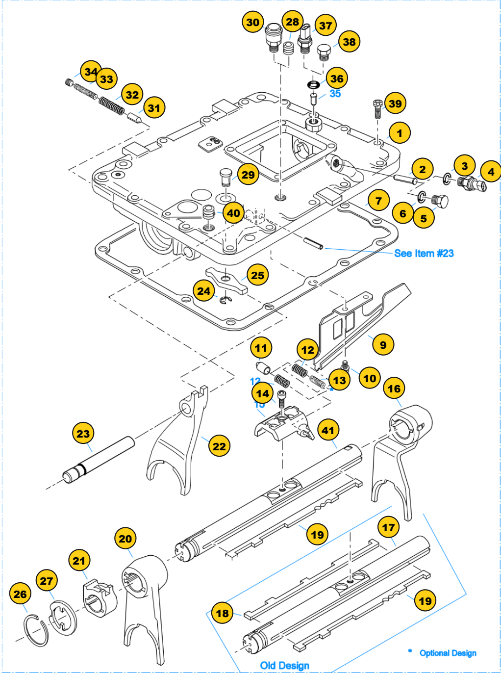
Group: SHIFT BAR HOUSING (FRO)
