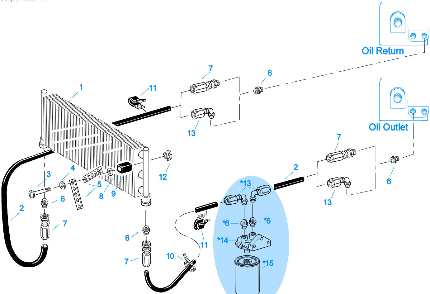
10526-9-94 Cooler C2
