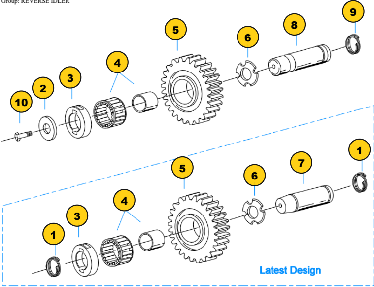
Group: REVERSE IDLER
