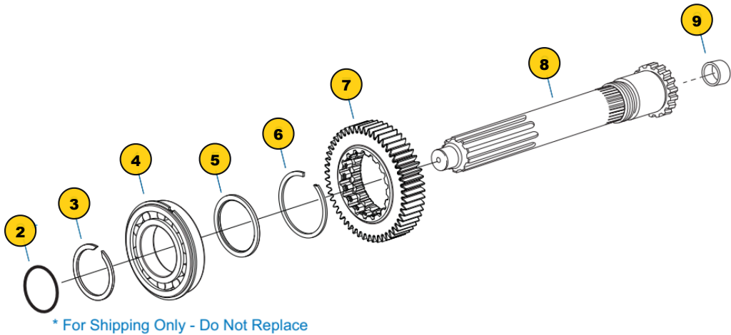
Group: INPUT SHAFT & DRIVE GEAR
